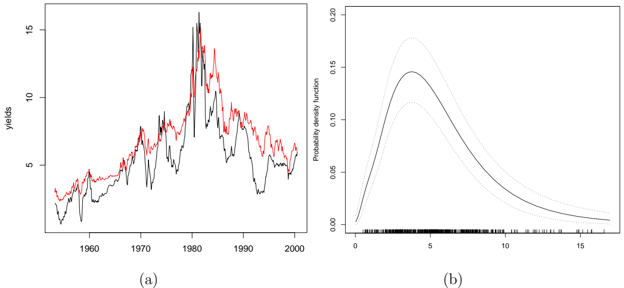
Figure 1: US sample: (a) time series of 3-month T-bill (in black) and 10-year yields; (b) short-rate density estimate.(The rug-plot at the basis of the density plot represents the frequency of the observations. Dotted lines are confidence bands.)
