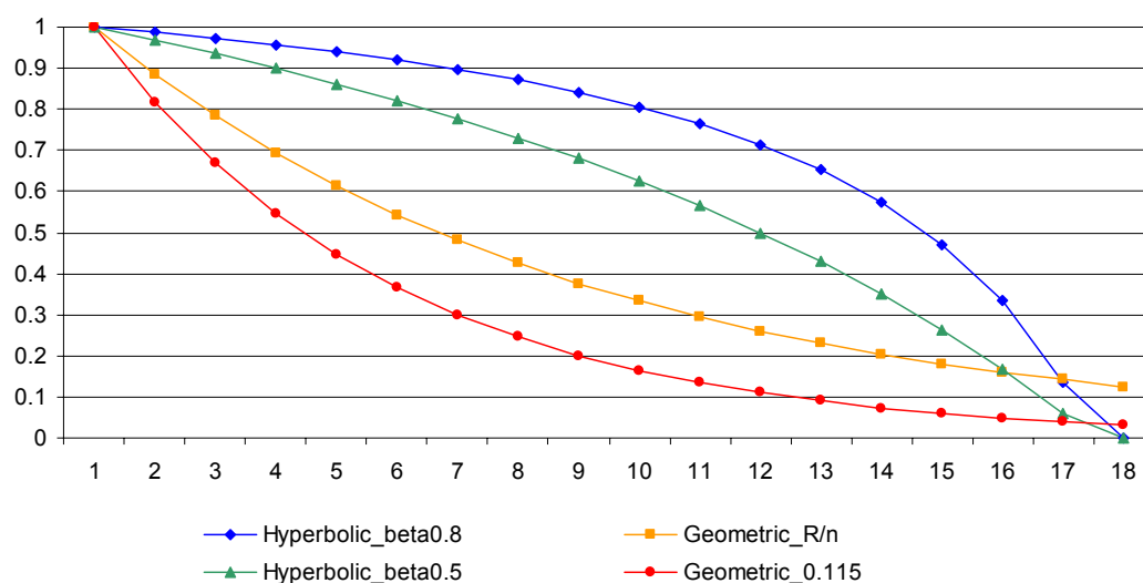
Figure 1: Hyperbolic and geometric age-efficiency patterns – Average service life 11 years
