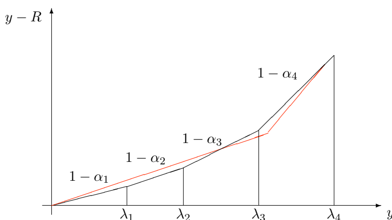
Figure 2: A piece-wise linear tax method defeating another. This figure illustrates a piece-wise linear tax method defeating a given one upon reducing the burden for low-income agents and increasing it for a small group of high-income agents.
