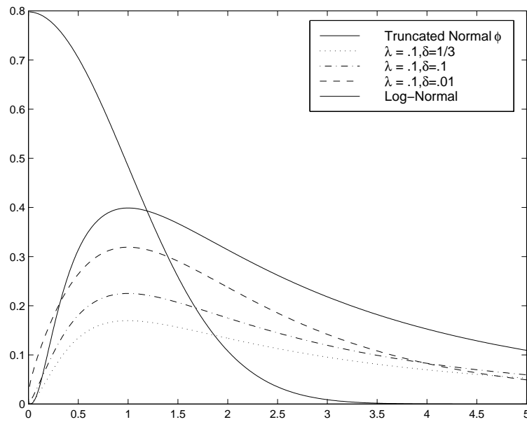
Figure 5: The densities of the log-normal, the truncated normal, and g_{\lambda,\delta} = DG_{\lambda,\delta} for various \delta , \lambda = .1 .
