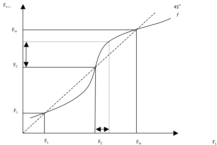
Figure 1: Recursion diagram
