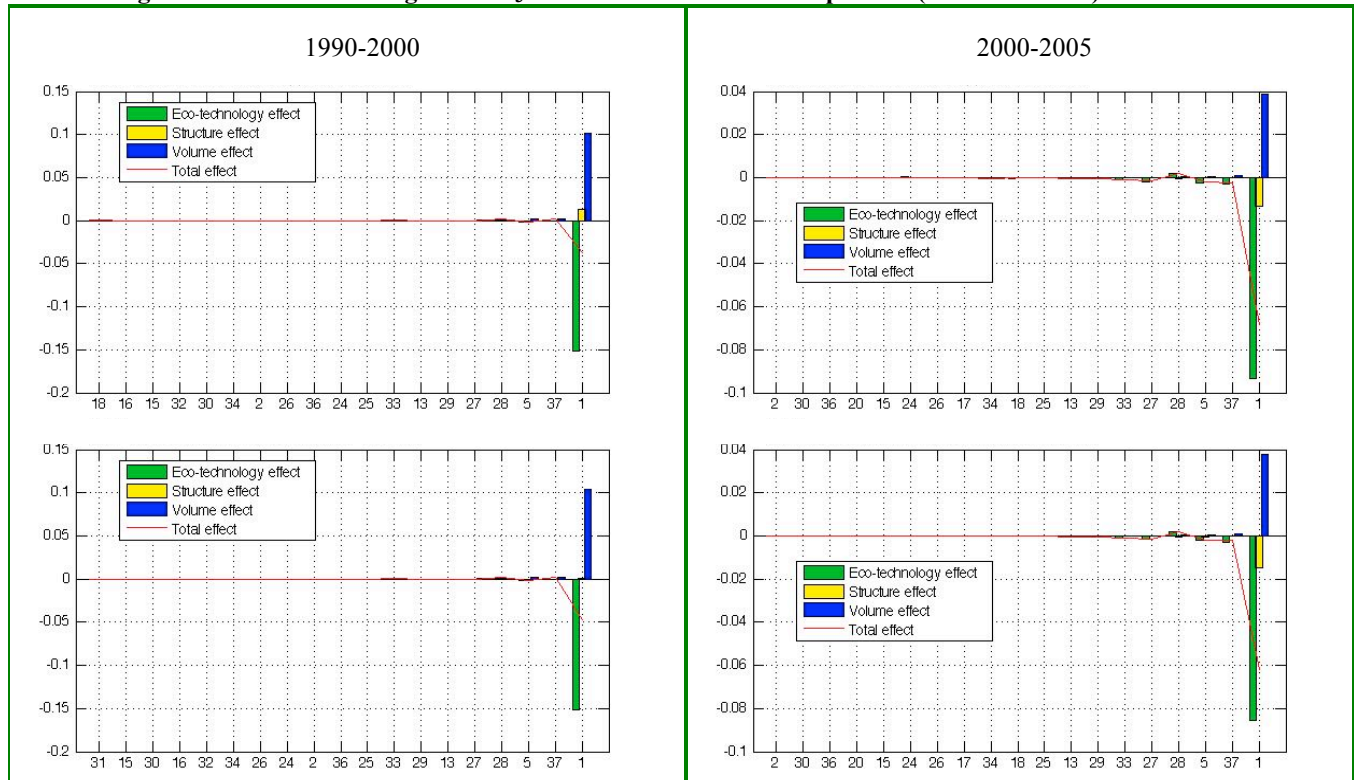
Figure D.6. SDA for changes in NH 3 emissions for the two sub-periods (PBA and CBA)
