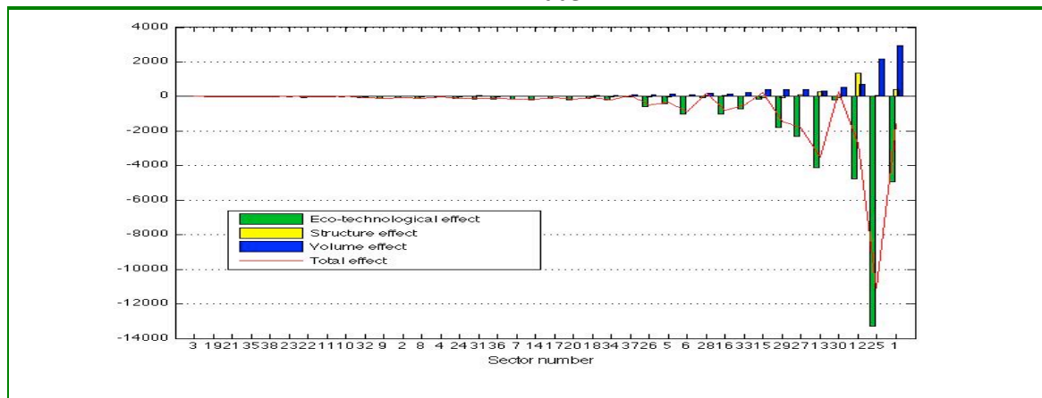
Figure 5. SDA for changes in acidification emissions index for the period 2000-2005
