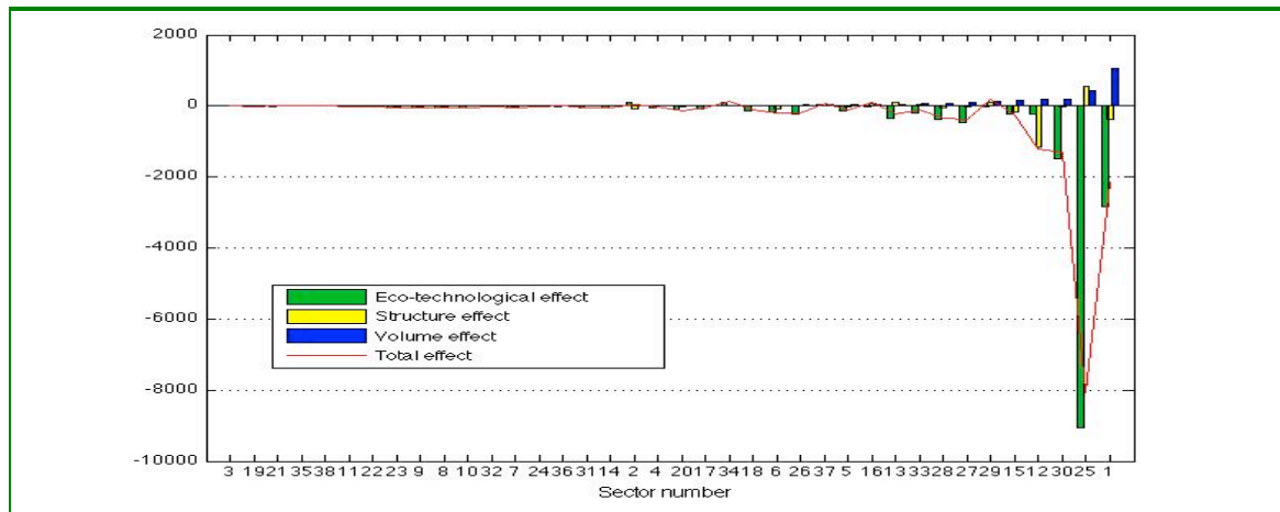
Figure 4. SDA for changes in acidification emissions index for the period 1995-2000
