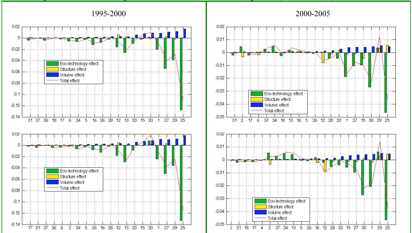
Figure D.4. SDA for changes in NO x emissions for the two sub-periods (PBA and CBA)
