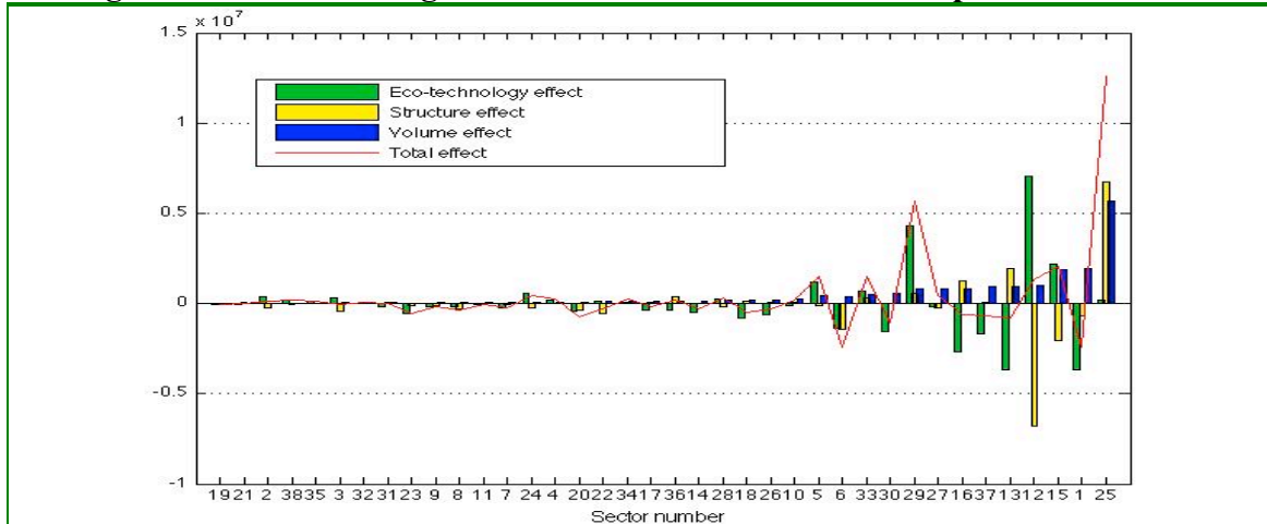
Figure 3. SDA for changes in GHG emissions index for the period 2000-2005
