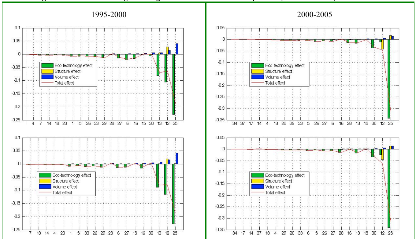
Figure D.5. SDA for changes in SO x emissions for the two sub-periods (PBA and CBA)
