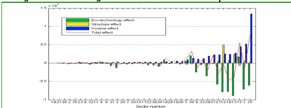
Figure 2. SDA for changes in GHG emissions index for the period 1995-2000
