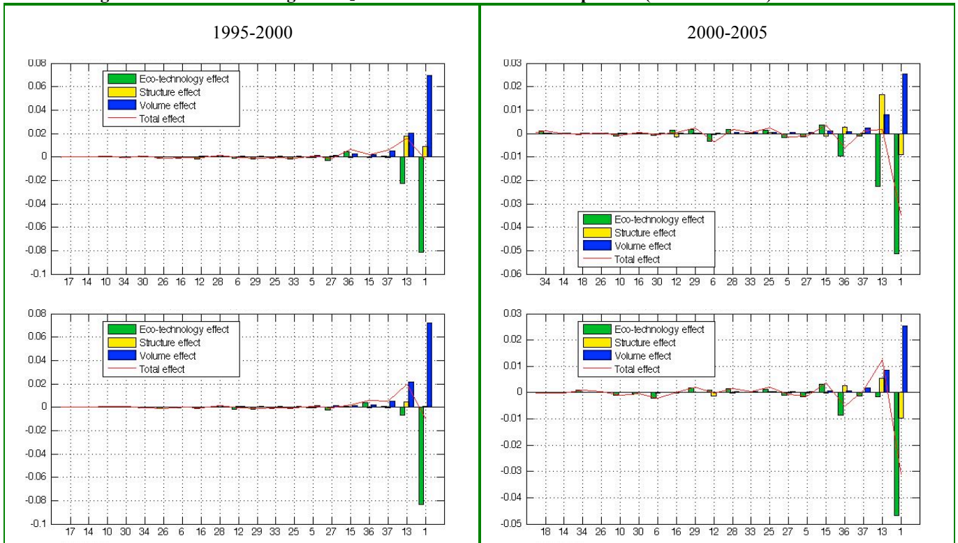
Figure D.2. SDA for changes in N 2 O emissions for the two sub-periods (PBA and CBA)
