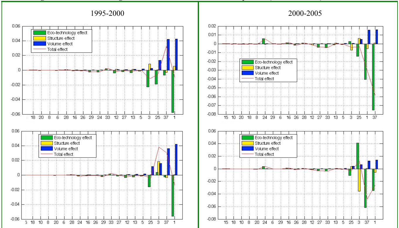
Figure D.3. SDA for changes in CH 4 emissions for the two sub-periods (PBA and CBA)
