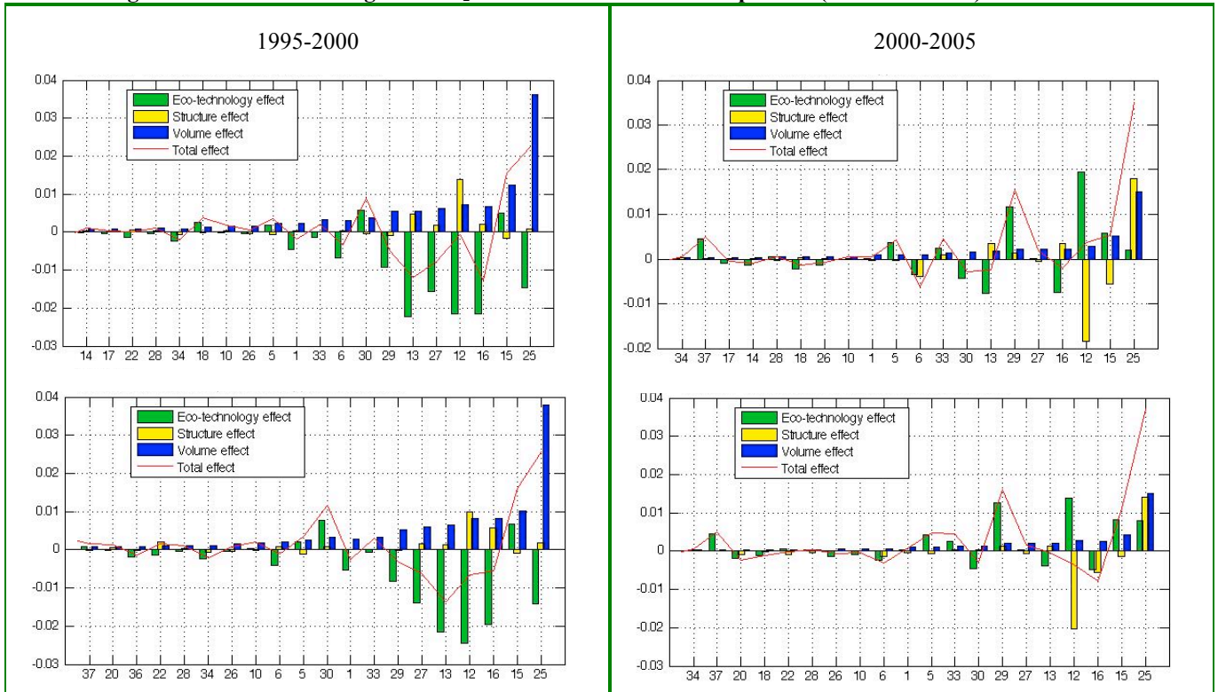
Figure D.1. SDA for changes in CO 2 emissions for the two sub-periods (PBA and CBA)
