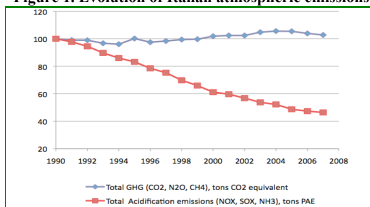
Figure 1. Evolution of Italian atmospheric emissions
