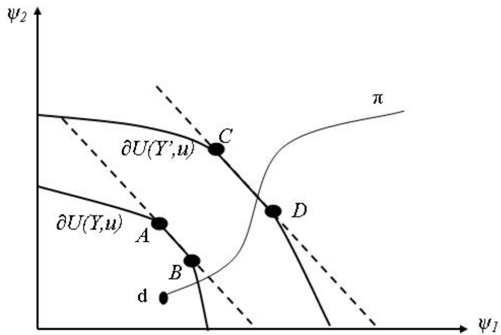
Figure 1: By Case 1, A < C and B < D .
