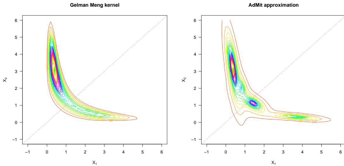
Figure 1: Left: contour plot of the kernel GelmanMeng . Right: contour plot of the four-component Student- t mixture approximation estimated by the function AdMit .
