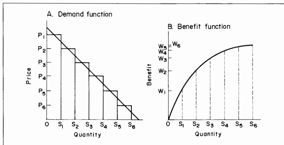
Fig. 3.3. Segmentation of demand and benefit functions for linear programming approximation (adapted from Duloy and Norton 1975).
