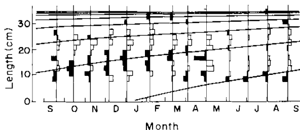
Fig. 4. Best fit of a von Bertalanffy growth curve to the length-frequency data for Hampala macrolepidota (after combining into 2 cm size groups and restructuring). The fit is obtained using the ELEFAN I program and yields estimates of K = 0.635 and L_{\infty} = 35.4 cm, with a "goodness-of-fit" of R_n = 0.209 .
