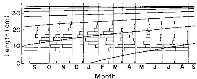
Fig. 5. Fit of the von Bertalanffy growth curve to the estimated true size frequencies of Hampala macrolepidota (as given in Table 12b; data combined into 2 cm size groups). Estimated K = 0.635 and L_{\infty} = 35.4 cm.
