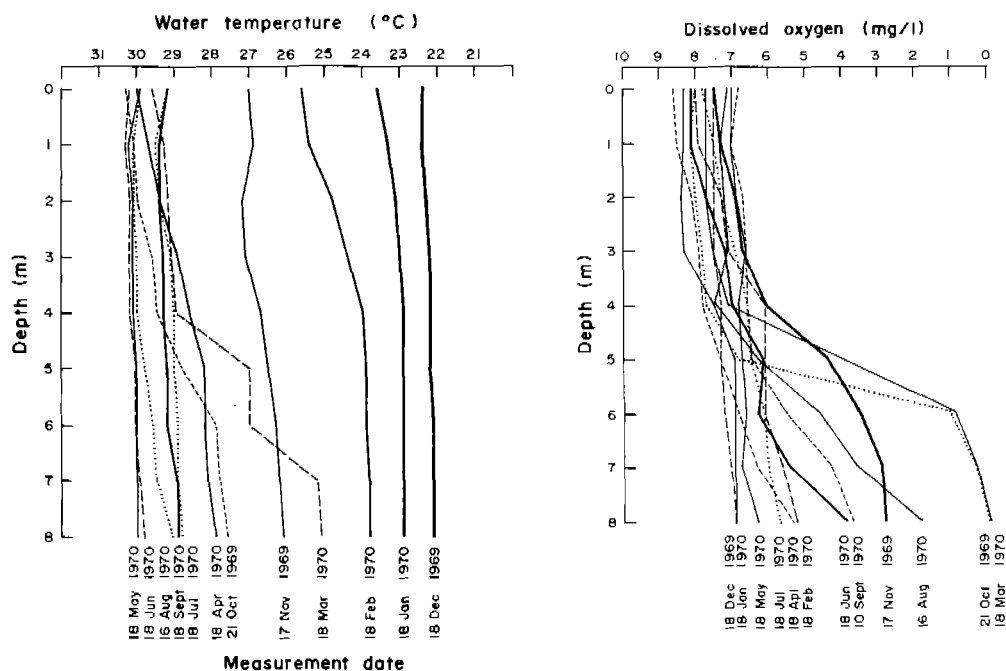
Fig. 2. Stratification of the water column in the Ubolratana Reservoir during wet and dry seasons, and associated dissolved oxygen concentrations (after Srisuwanataj 1970).
