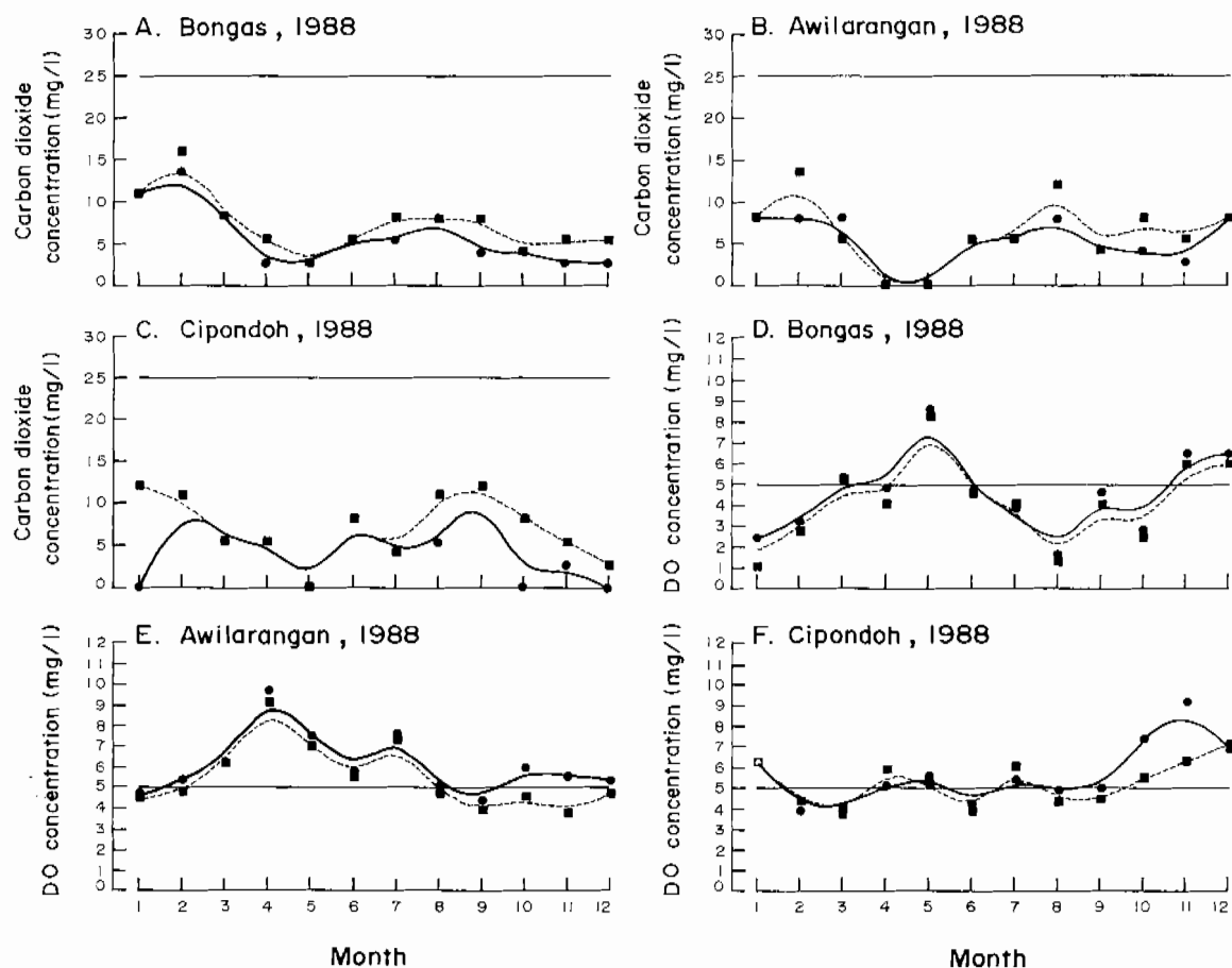
Fig. 4. Early morning (0600 hours) water quality at two depths for three stations in the Saguling Reservoir with significant cage experimental (Awilarangan and Cipondoh) or commercial (Bongas) operations over a 12-month period in 1988. Dashed lines and closed boxes are water quality readings at 2.0 m depth, and the closed circles and dark lines water quality parameters at 0.2 m depth.
