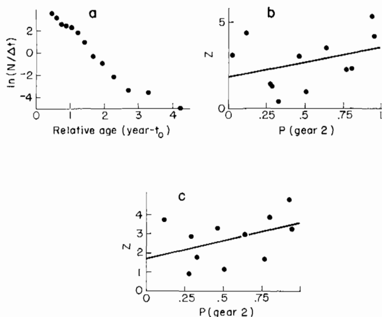
Fig. 7. Output of the ELEFAN IV computer program for the estimation of natural mortality rates. a. Length-converted catch curve indicating age- or size-specific changes in mortality rates, based on estimated true size frequencies (in 2 cm size classes) of Hampala macrolepidota in the Saguling Reservoir. b. Regression of estimated total mortality rates of successive size classes against the probability of capture in the small-scale gill net fleet using Munro's method. M = 1.789 ; S.E. = 0.892; Z = 1.789 + 1.75 P . c. As in Fig. 7b, using Moreau's method. M = 1.729 ; S.E. = 0.835; Z = 1.729 + 1.83 P .
