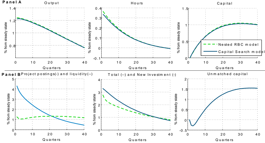
Figure 2: IRFs to a persistent technology shock for baseline specification
