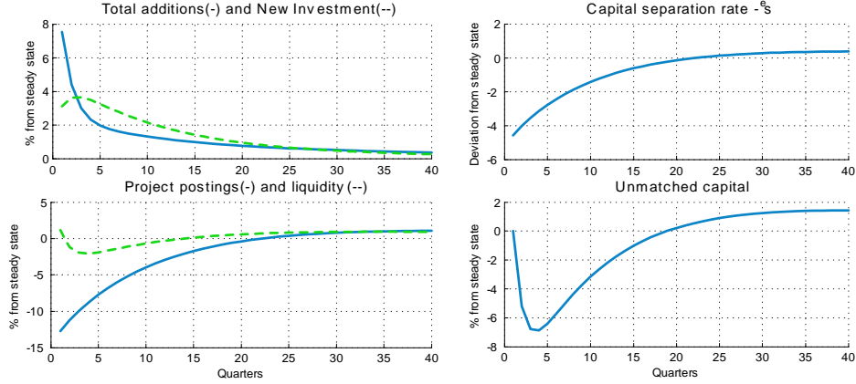
Figure 4: IRFs to a persistent technology shock for the extended model.
