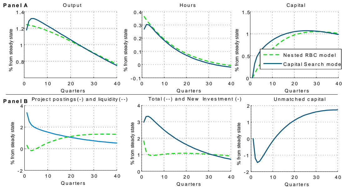
Figure 3: IRFs to a persistent technology shock for counterfactually high separation rate
