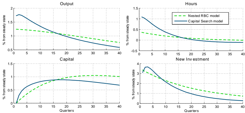
Figure 3: IRFs to a persistent technology shock for the extended model
