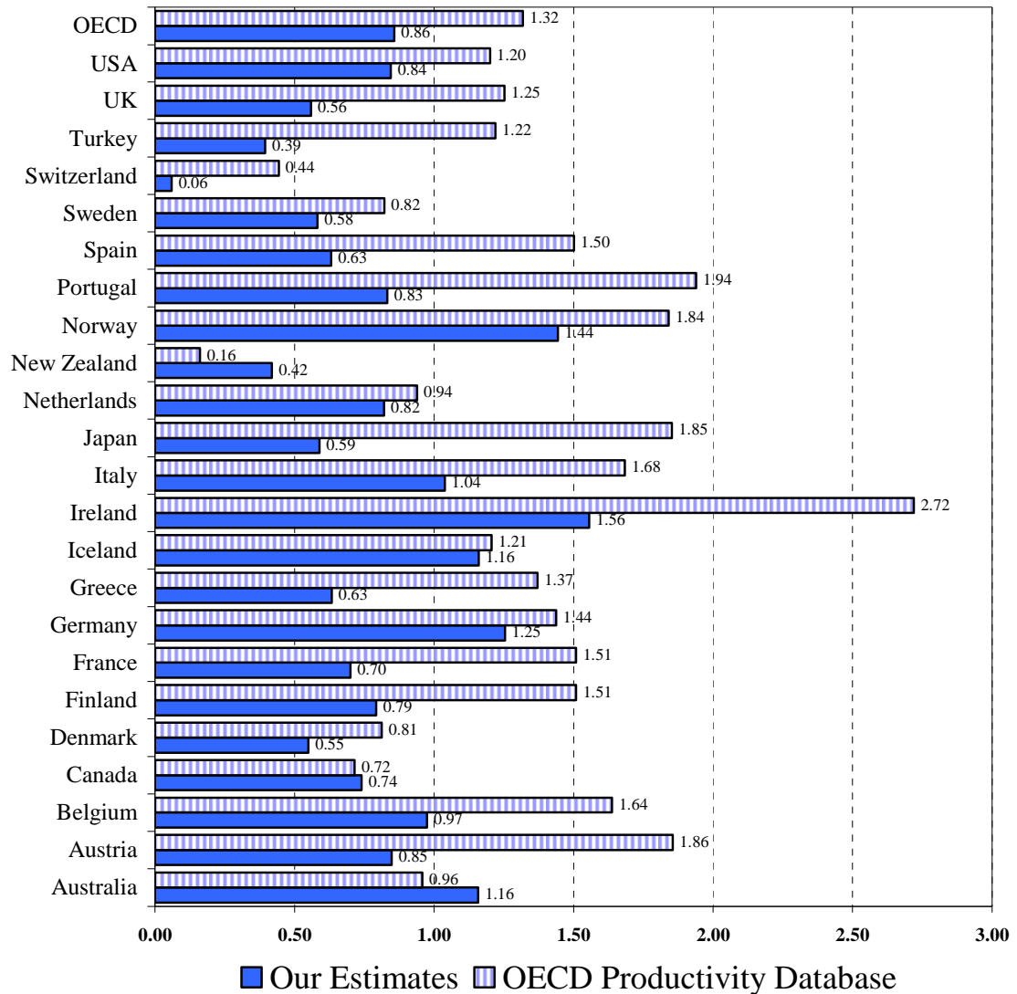
Figure 2 – TFP Growth (%), 1960-2003
