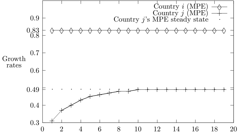
Figures 4a and 4b: different balanced growth rates
