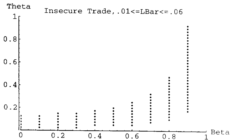
Figure 3. Parameters Supporting Interior Equilibria
