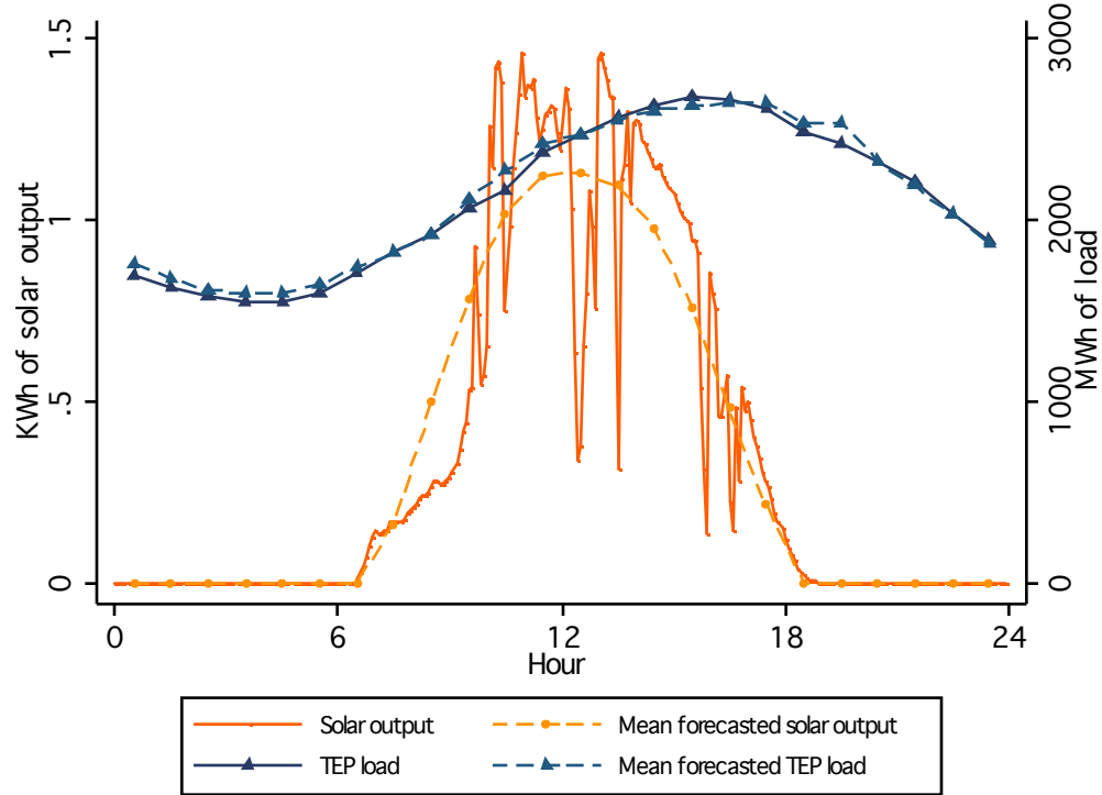
Figure 2: Predicted and actual southeastern Arizona load and solar output, Aug. 15, 2008
