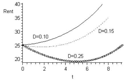
Figure 4: Rent function for D = 0.1 (solid line), D = 0.15 (dotted line), and D = 0.25 (in circles).
