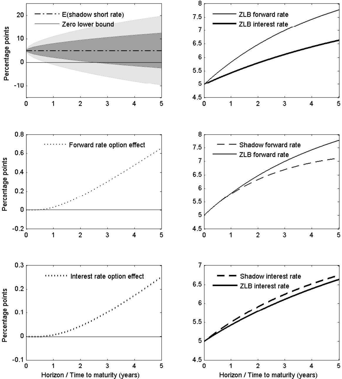
Figure 3: Perspectives on the ZLB-GATSM(2) term structure with s_1(t) = 0.05 and s_1(t) = -0.00 , so r(t) = 5 percent.
