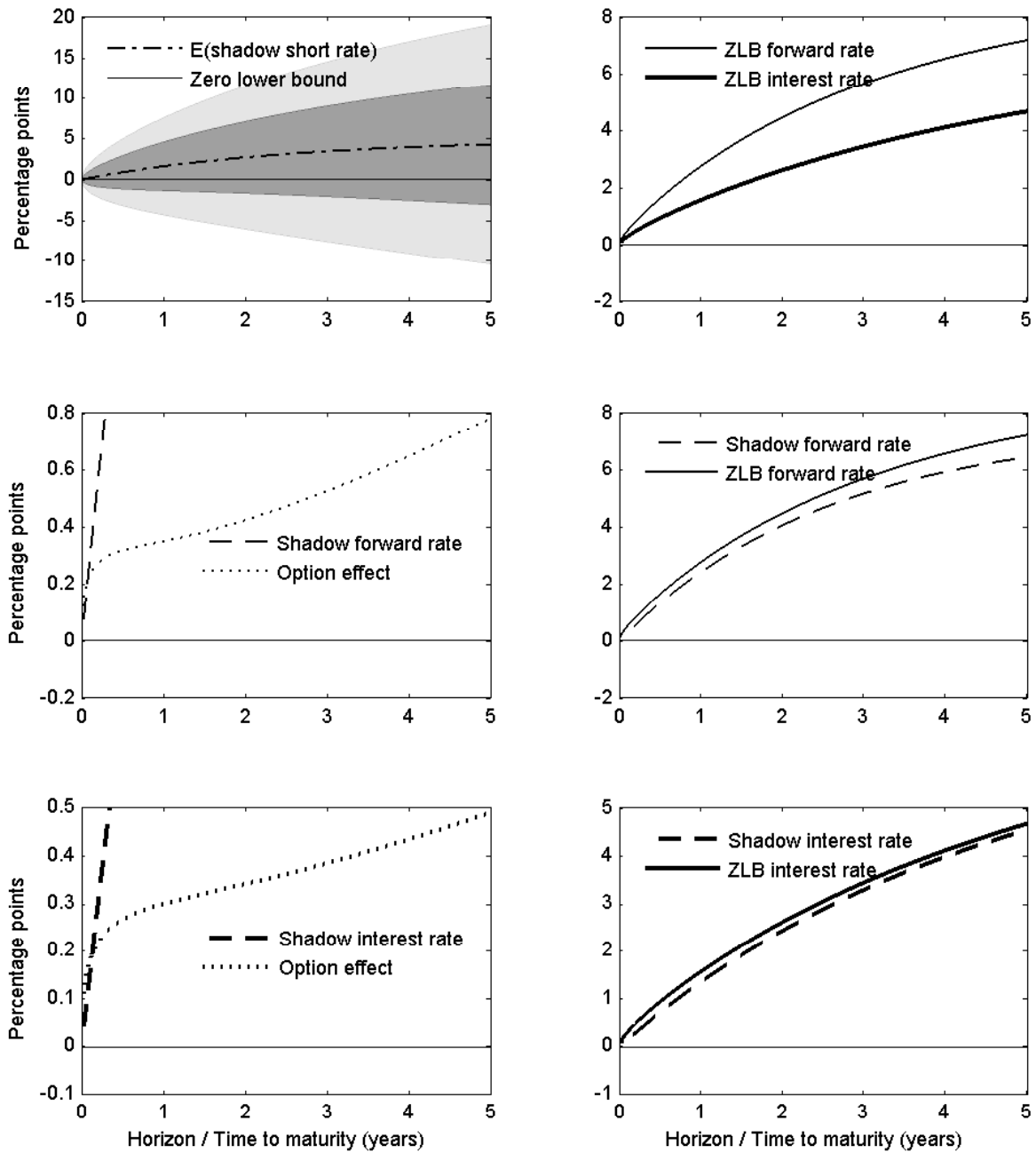
Figure 2: Perspectives on the ZLB-GATSM(2) term structure with s_1(t) = 0.05 and s_1(t) = -0.05 , so r(t) = 0 percent.
