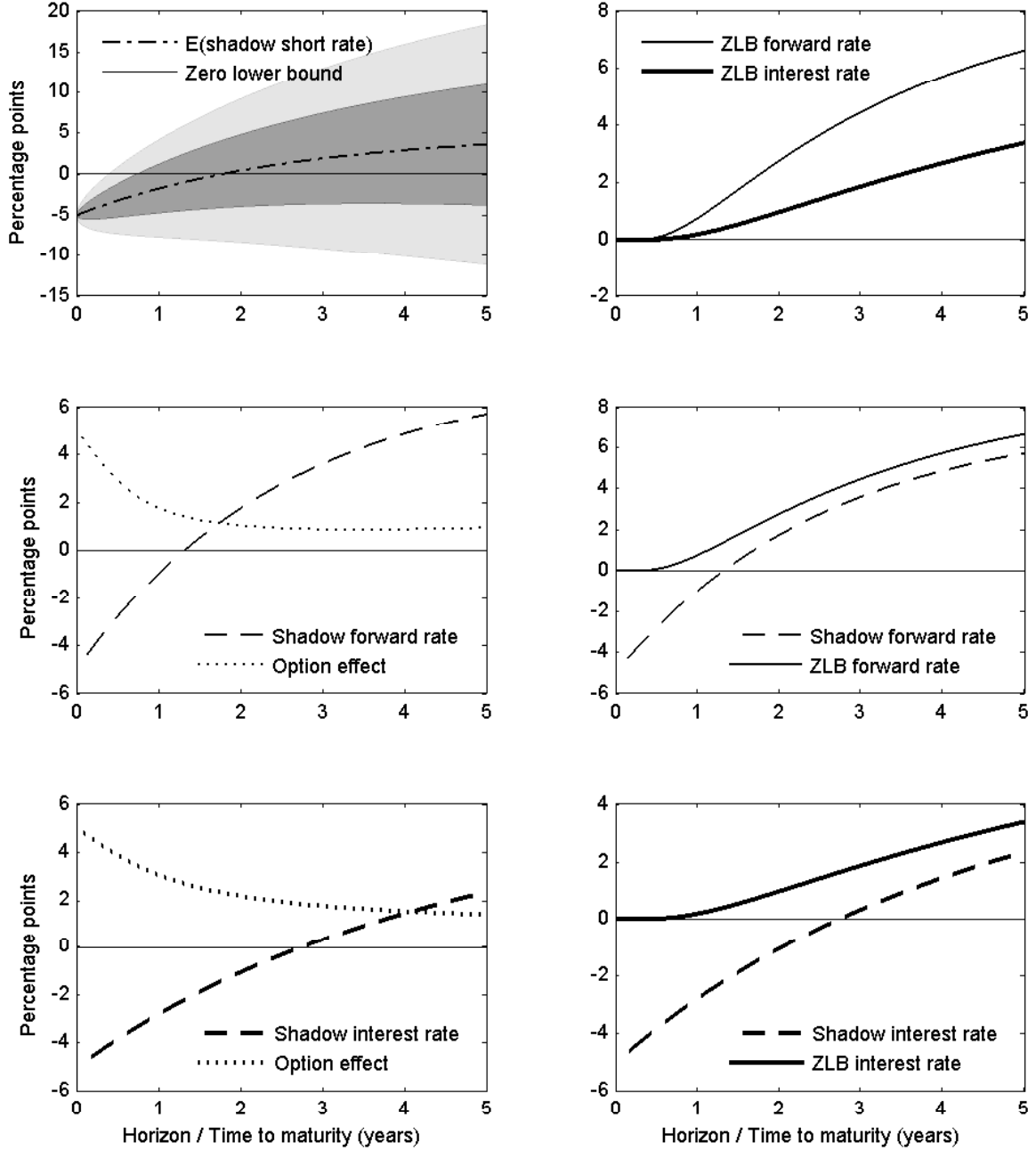
Figure 1: Perspectives on the ZLB-GATSM(2) term structure with s_1(t) = 0.05 and s_1(t) = -0.10 , so r(t) = -5 percent.
