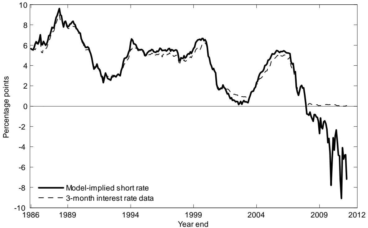
Figure 7: The 3-month interest rate data and estimates of the ZLB-GATSM(2) shadow short rate r(t) = s_1(t) + s_2(t) .
