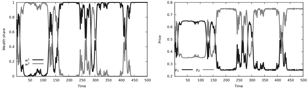
Figure 6: Price and wealth dynamics for the market represented in the right panel of Fig. 4. Left panel: typical wealth dynamics. Right panel: typical price dynamics.
