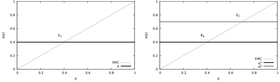
Figure 1: Left Panel: EMC plot representing a market with a single investor with \alpha = 0.4 . The only possible outcome of the dynamics is E_1 . Right Panel: EMC plot representing a two-agent market. Investment shares are \alpha^1 = 0.4 and \alpha^2 = 0.7 respectively. E_1 and E_2 are the two single survivor long-run equilibria.
