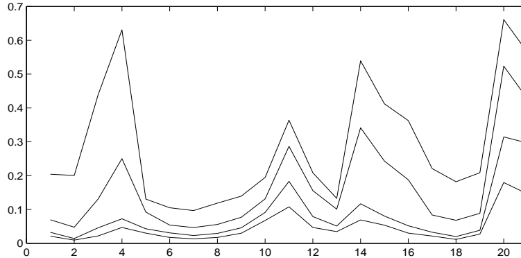
The four lines, from top to bottom, correspond to the frequency band [0, \rho] , with \rho taking the values \pi, \pi/4, \pi/16, \pi/32 . The variables, indicated in this Figure, as well as in Figures 4.1, 5.1, 5.2, by numbers from 1 to 21 are fcp1, fcp3, nfcpl, nfcps, t1, t3, t5, t7, t10, t20, tb3, tb6, tb12, ed1, ed3, ed6, cd1, cd3, cd6, ffr, rp .
