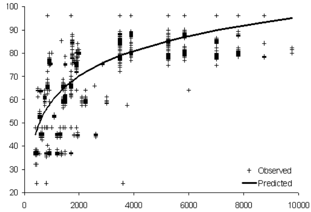
Figure 2. Relationship between Road Capacity and Free-Flow Speed
