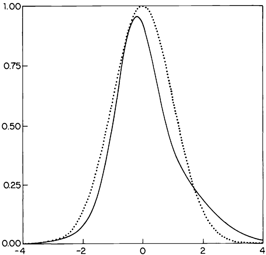
Fig. C2.1 Standardized (zero mean and unit variance) distribution with zero and unit skewness, respectively.
