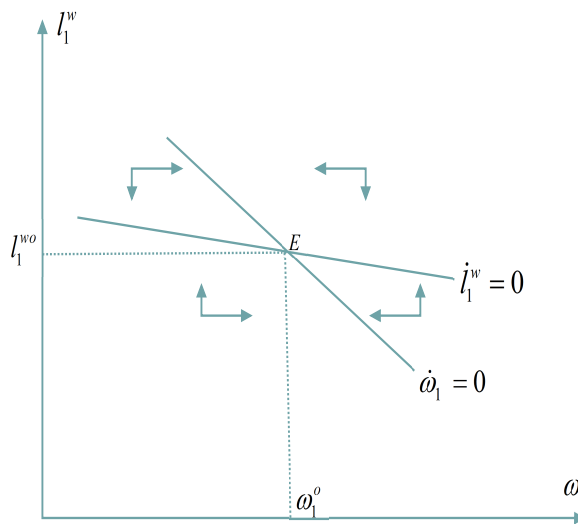
Figure 2: The case of a large parameter \beta_e
