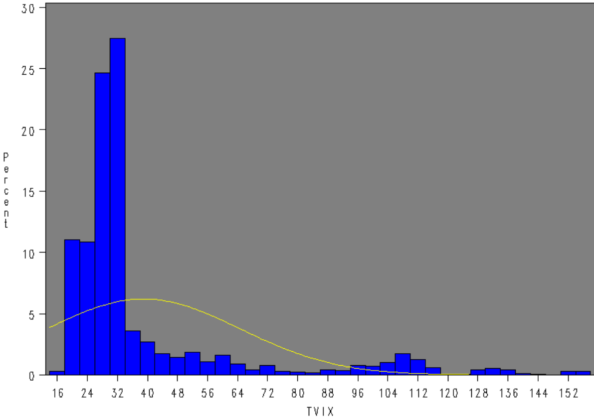
Figure 3.4: TVIX histogram
