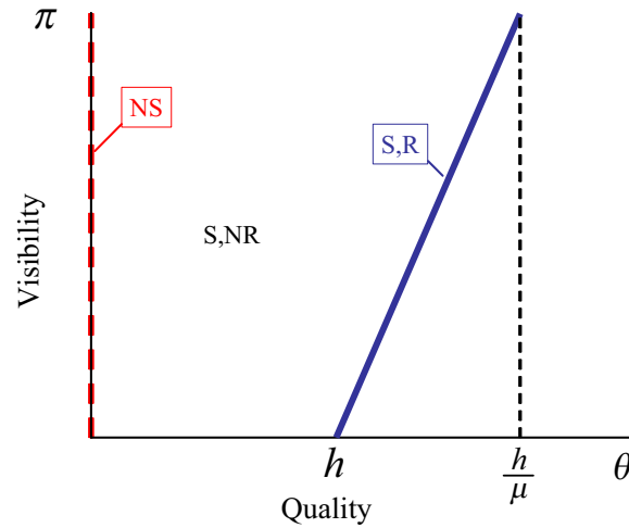
Figure 1: Graphical representation of strategies in the (\theta, \pi) space.
