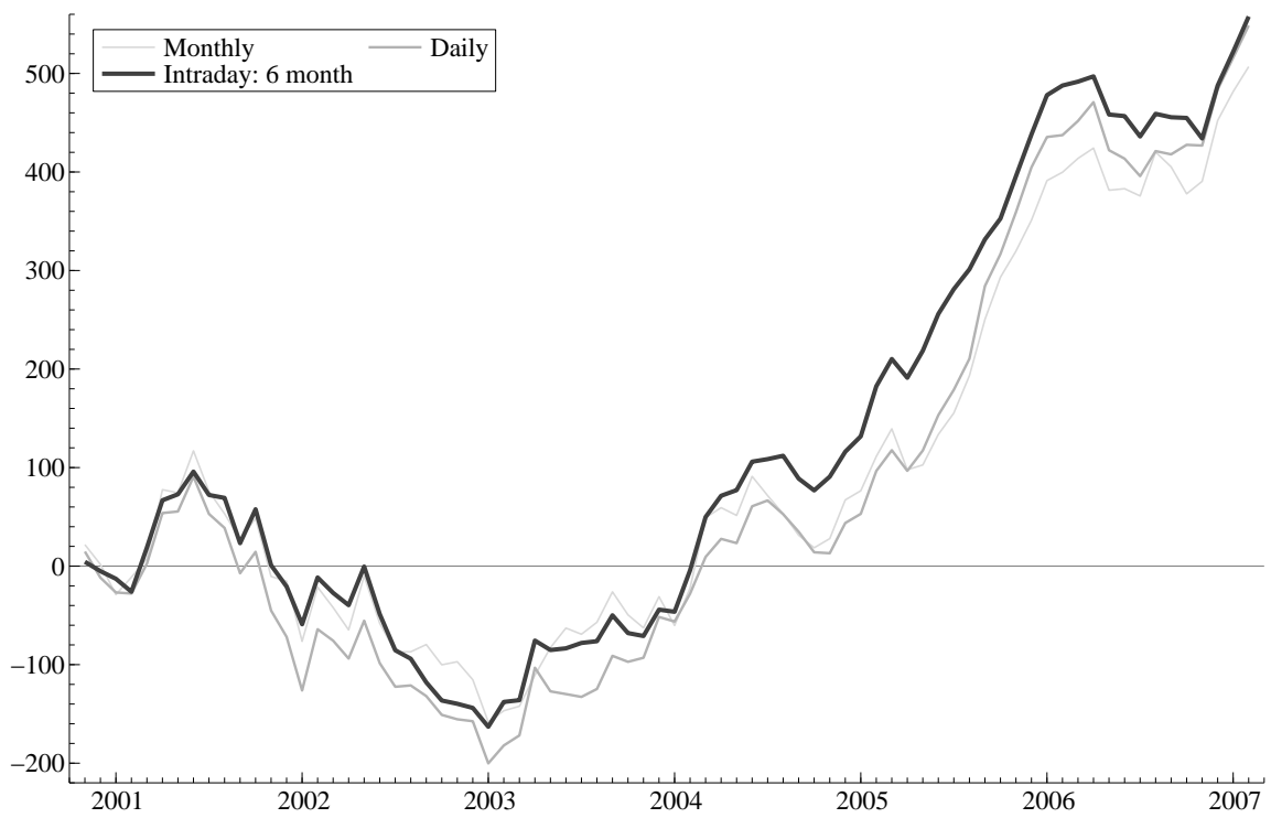
Figure 1: Cumulative portfolio returns
