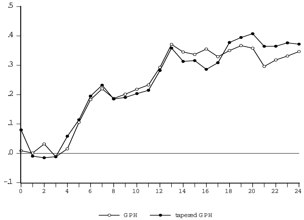
Figure 2: \hat{d}_t and \hat{d}_{TA} estimates of the constructed series x_t - y_{t-l} where l = 0, \dots, 24 (horizontal axis) and x_t, y_t denote the Austrian and German ex-post real interest rates respectively. The zero line is also displayed.
