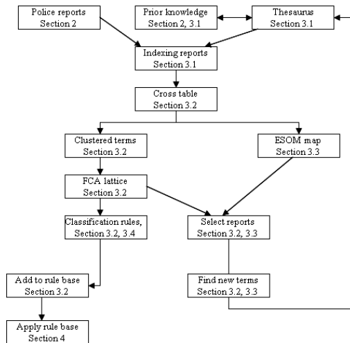
Figure 1: Knowledge acquisition process
