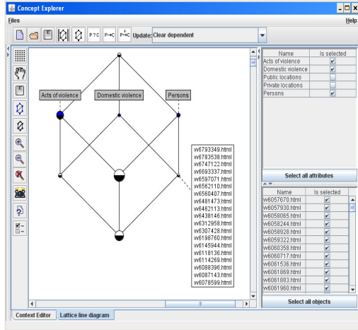
Figure 6: Lattice with case numbers
