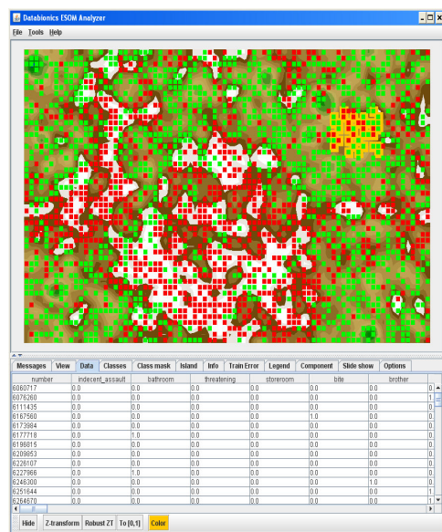
Figure 7. Toroidal ESOM trained on the thesaurus from section 3.1
