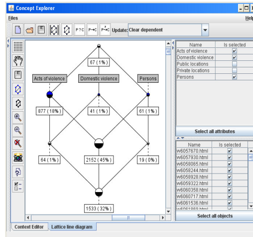
Figure 5: Lattice with own object count
