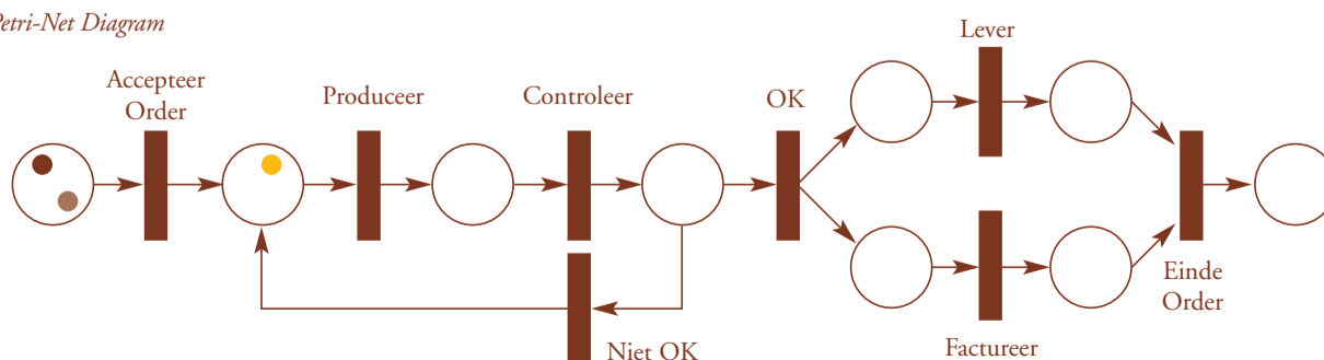
Petri-Net Diagram
