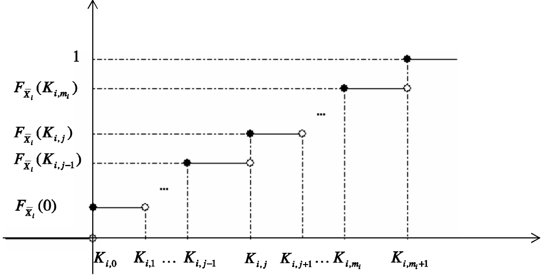
Figure 1: The cdf of \bar{X}_i .
