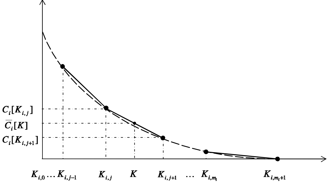
Figure 2: The functions \bar{C}_i[K] and C_i[K] .
