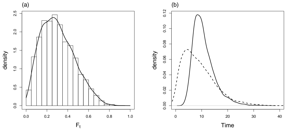
Figure 2: (a) Histogram and density estimates of the posterior distribution of F_t for t = 5 . (b) Density estimate of I_T(\tilde{\mu}^*) (—) and I_T(\tilde{\mu}) (- - -) for T = 50 ; sample mean and sample s.d. of I_T(\tilde{\mu}^*)
