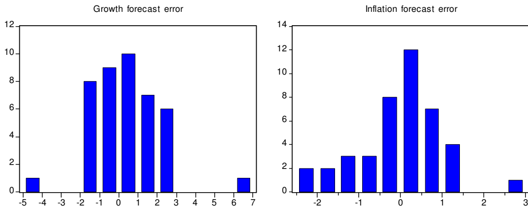
Figure 2: Histograms
