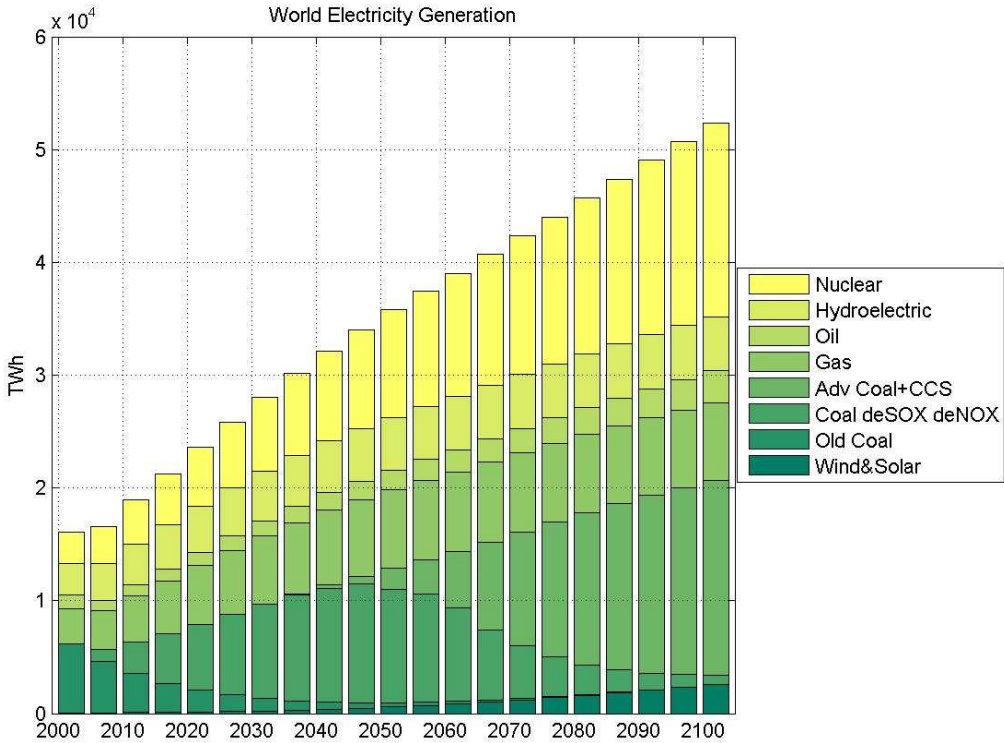
Figure 11: Power Generation Mix in the Cooperative Solution
