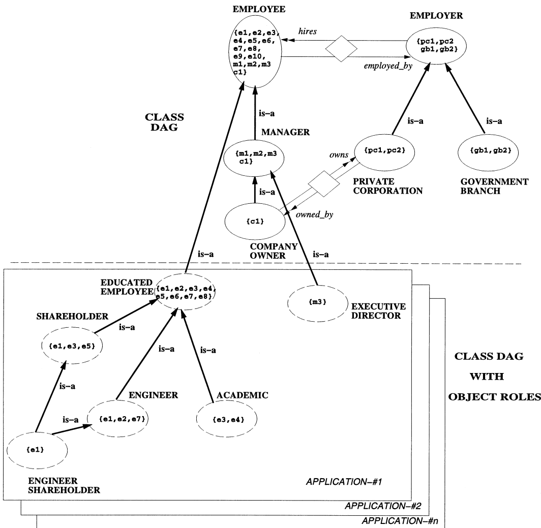
Fig. 4. The class hierarchy for the type schema in Fig. 2 evolved with roles
