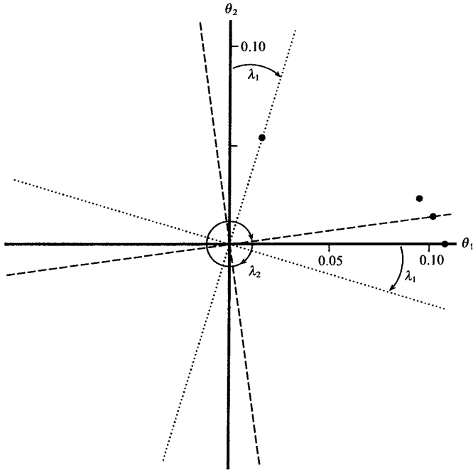
FIGURE 2 Factor rotation
