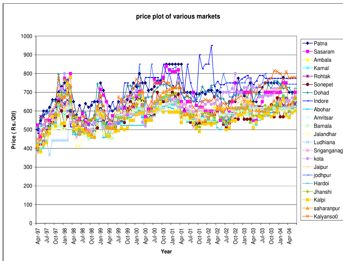
Figure 10: Wheat price data for 22 markets, April 1997 to June 2004
