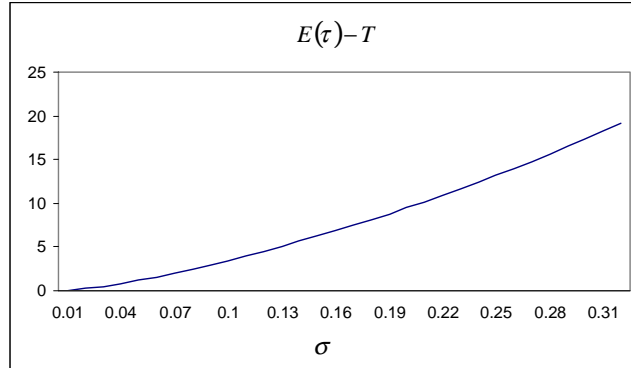
Figure 3: E(\tau) - T as a function of \sigma
