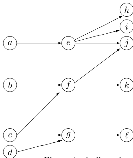
Figure 1: A digraph.
