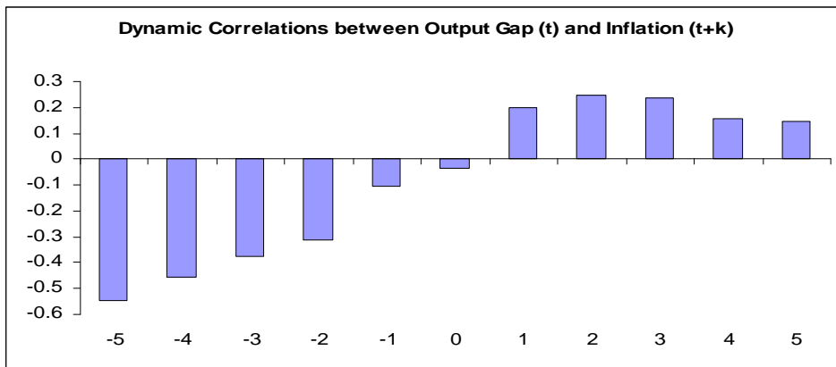
Fig. 1. Dynamic Correlations
