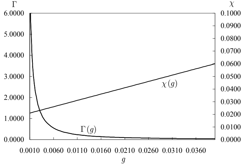
FIGURE 1: EXISTENCE AND UNIQUENESS OF POSITIVE SOLUTION
