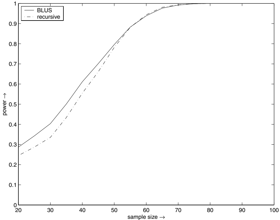
Figure 7. BLUS and recursive residuals compared: Quandt's simulated data.
