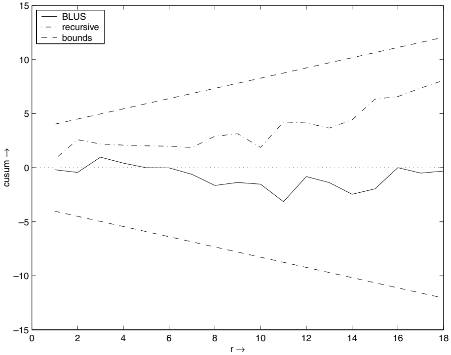
Figure 3. Cusum plots: Quandt's data.
