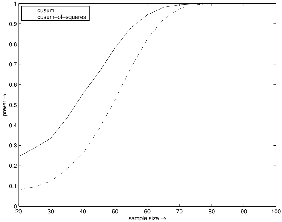
Figure 6. Power of recursive residuals: Quandt's simulated data.
