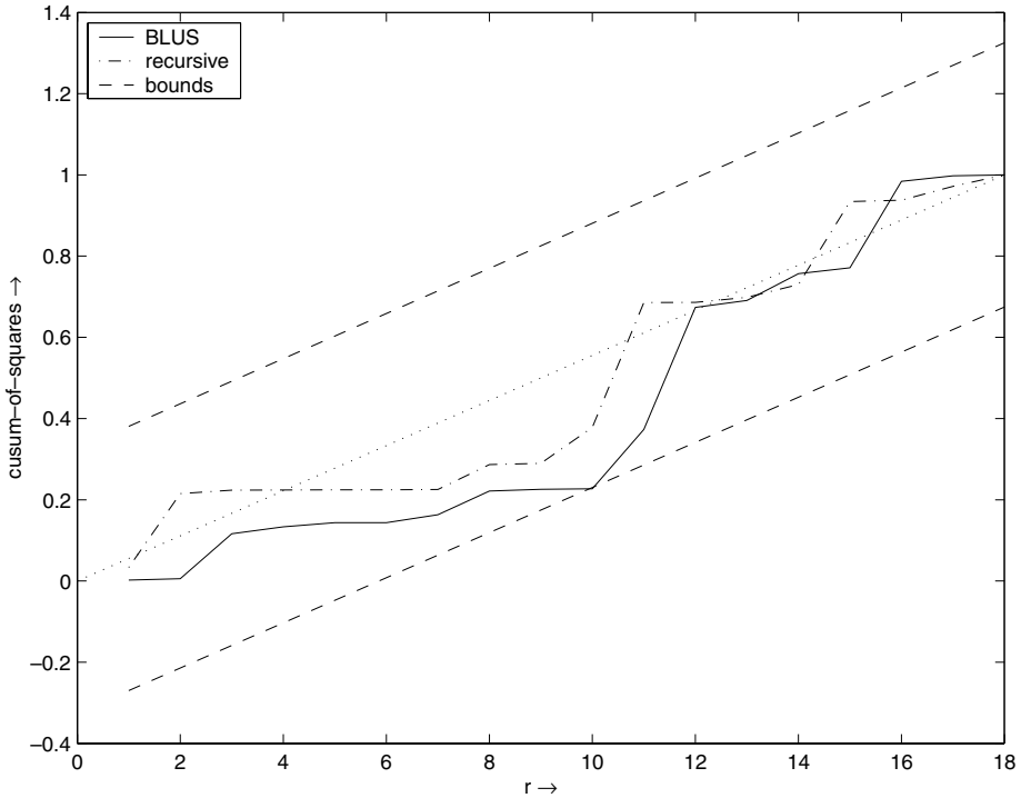
Figure 4. Cusum-of-squares plots: Quandt's data.
