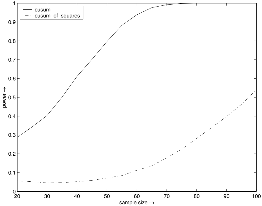
Figure 5. Power of BLUS residuals: Quandt's simulated data.
