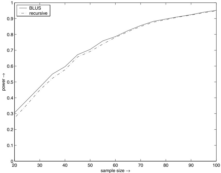
Figure 1. Power of two-sided F -test: Theil's simulated data.
