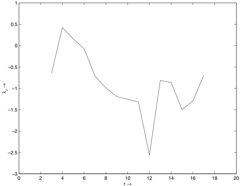
Figure 2. Quandt's likelihood ratio \lambda_r .
