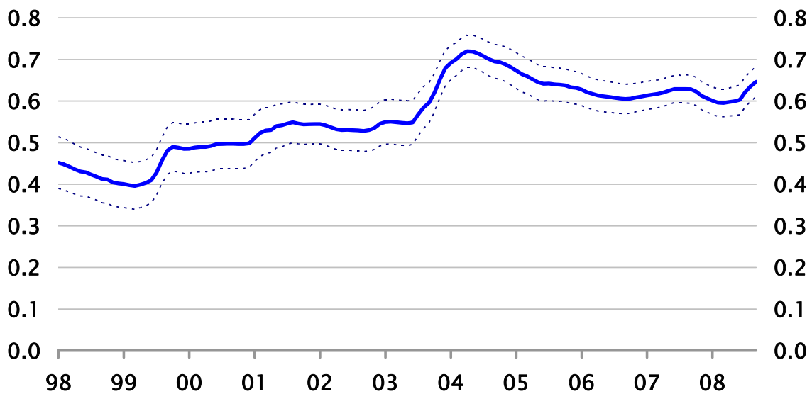
Figure 5 Pass-through to Wholesale Import Price (10-year rolling regression)
