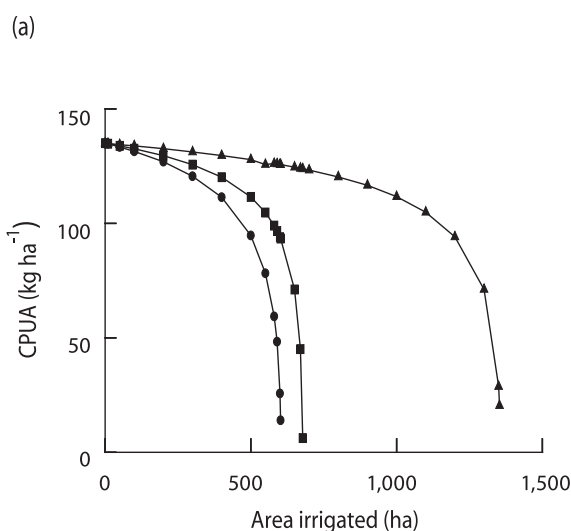
FIGURE 12a. The effect of dry season irrigation for boro rice on fish production in Bangladeshi floodplains measured in terms of catch per unit area (CPUA). Figure 12b. Predicted yield of P. sophore as a function of dry season area relative to flood season area.
