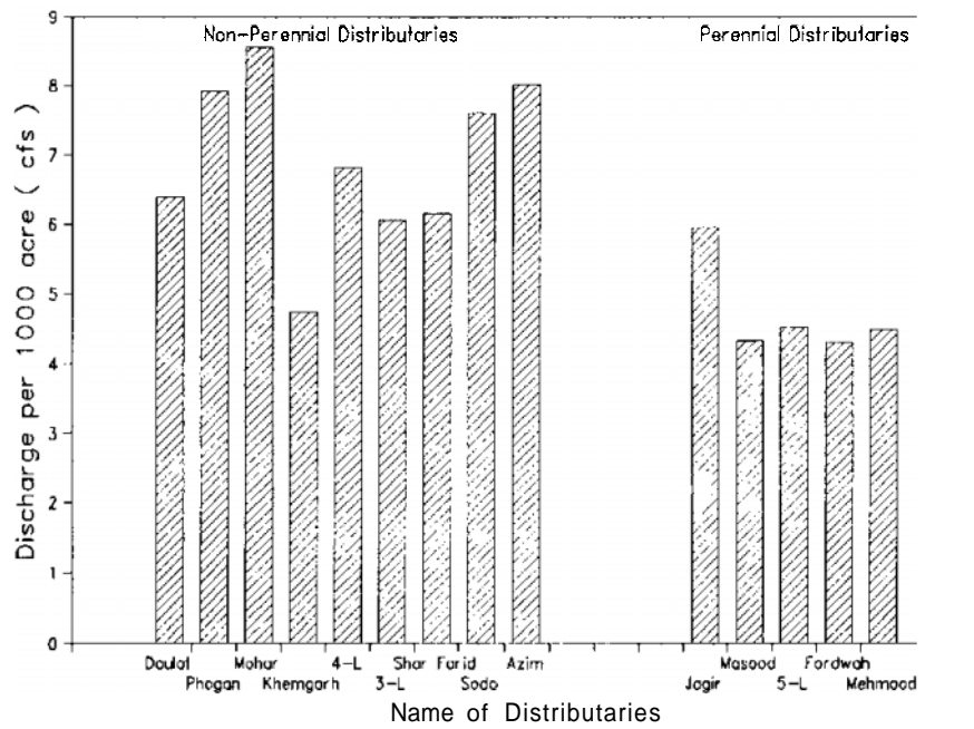
Figure 2.1. Design discharge at the head of distributaries in Chishtian Sub-division.
