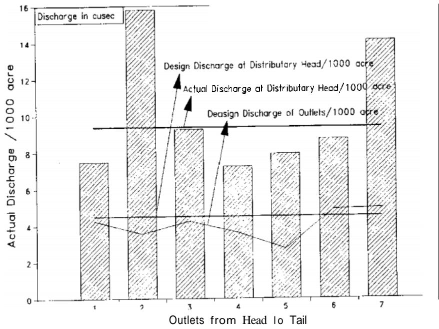
Figure 2.13. Normalised discharges of Mehmood Distributary and outlets.
