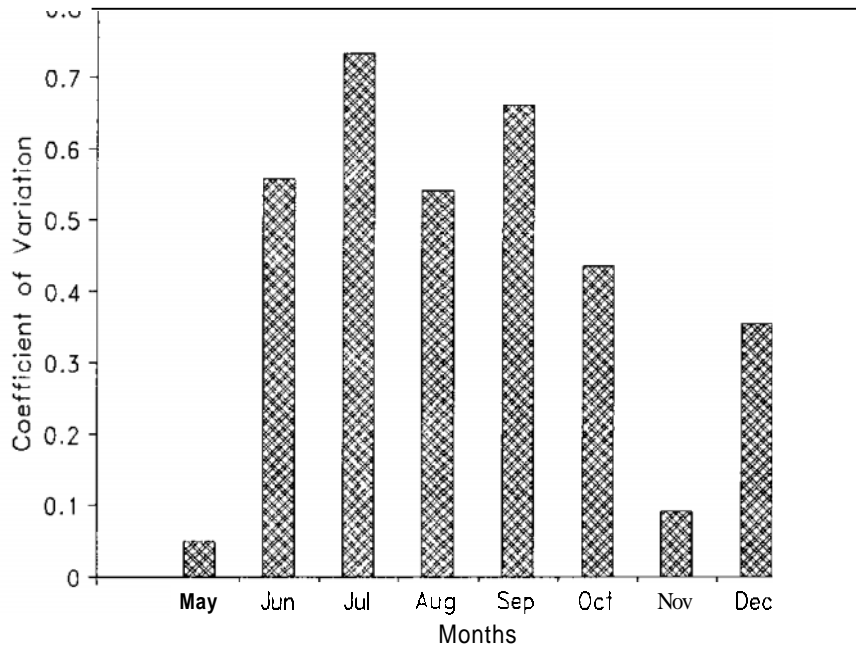
Figure 3.1. Temporal coefficient of variation at Fordwah Distributary head, 1992.
