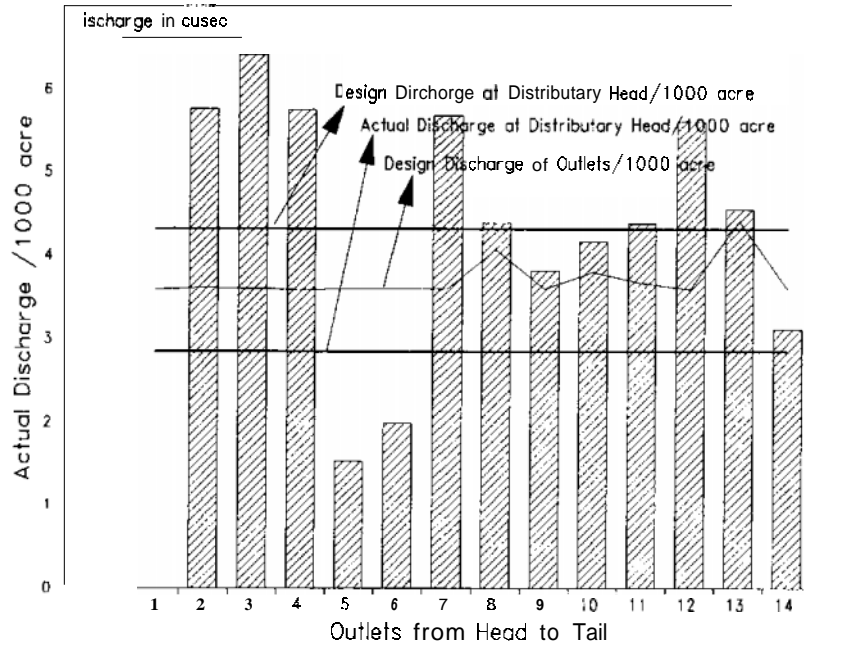
Figure 2.10. Normalised discharges of Masood Distributary and outlets.
