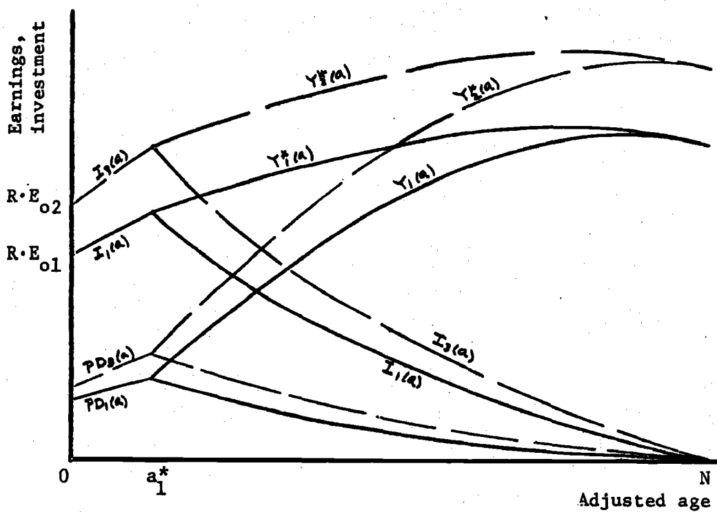
Figure 5. Changes in observed income and investment paths due to changes in E_0 and \beta which leaves a^* unaltered
