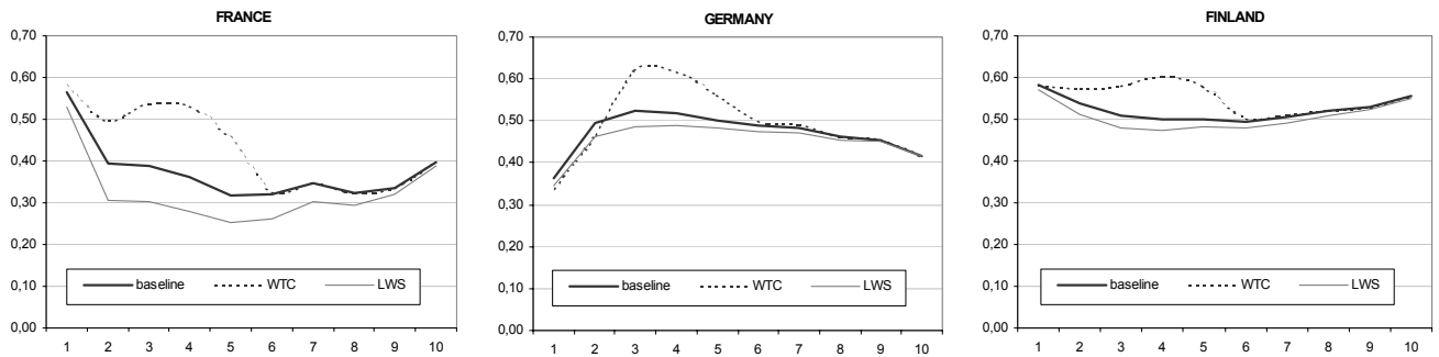
Figure 20: Distribution of EMTRs per decile of disposable income per adult equivalent
