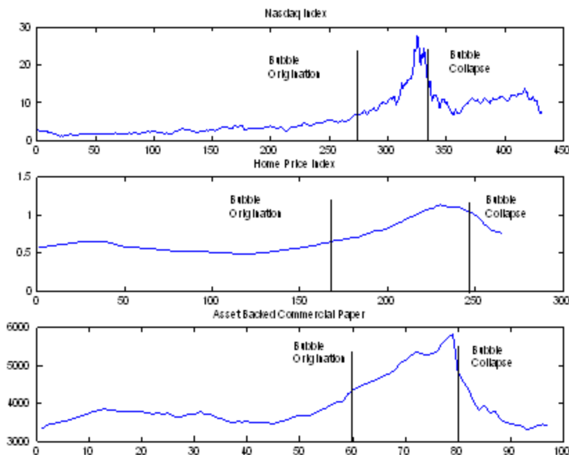
Figure 1: Time series plots of real prices for three financial assets: monthly observations on the Nasdaq index from February 1973 to January 2009; monthly observations on the house price index from January 1987 to January 2009; monthly observations on the outstanding value of asset backed commercial paper from January 2001 to January 2009. All series are normalized by the CPI. The estimated bubble origination and collapse dates are also shown on the figures.
