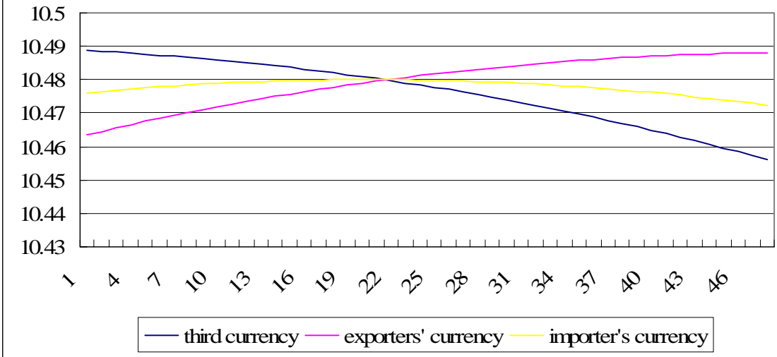
Figure 1-a. Comparison of Each Expected Utility: \mu = 5
