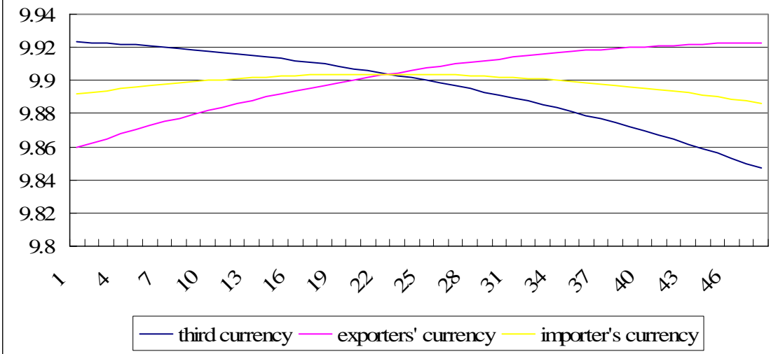
Figure 1-b. Comparison of Each Expected Utility: \mu = 7.5
