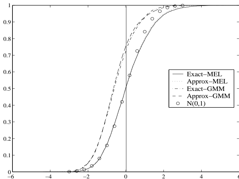
Figure 2: n - K = 100, K_2 = 10, \alpha = 1, \delta^2 = 100
