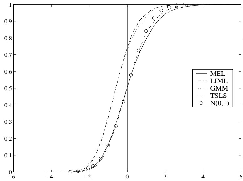
Figure 3: CDF of Standardized estimators: n - K = 100, K_2 = 10, \alpha = 1, \delta^2 = 100
