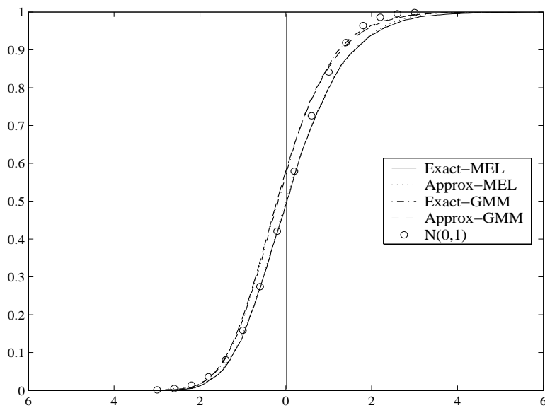
Figure 1: n - K = 30, K_2 = 3, \alpha = 1, \delta^2 = 50
