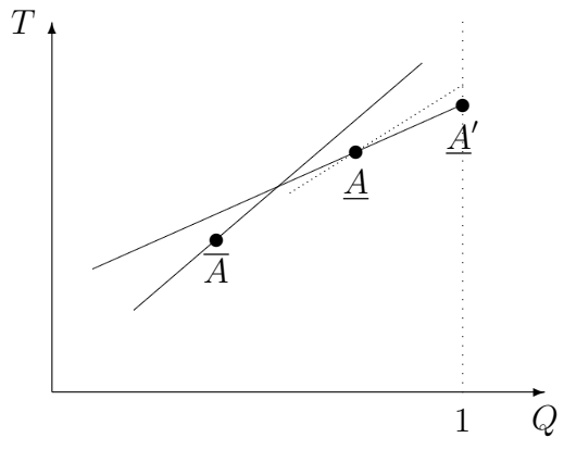
Figure 2 Attracting type \underline{\theta} by pivoting around (\underline{Q}, \underline{T})
