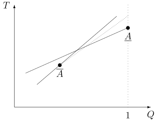
Figure 3 Attracting type \underline{\theta} by pivoting around (\overline{Q}, \overline{T})
