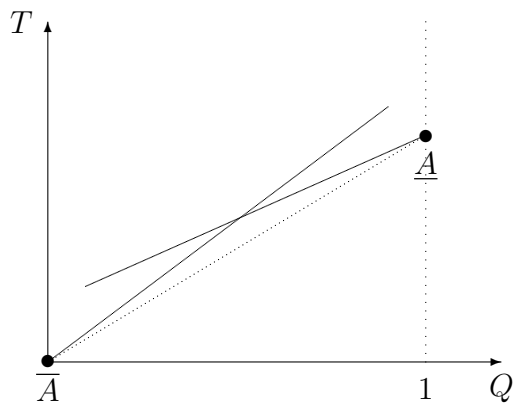
Figure 6 Aggregate equilibrium allocations when \mathbf{E}[v(\theta)] < \bar{\theta}
