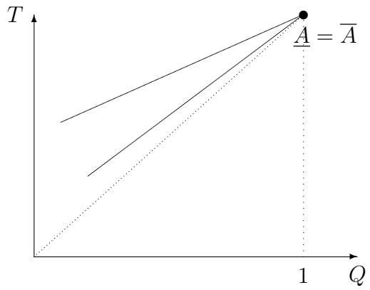
Figure 5 Aggregate equilibrium allocations when \mathbf{E}[v(\theta)] > \bar{\theta}
