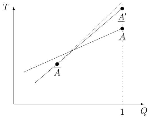
Figure 4 Attracting both types by pivoting around (\bar{Q}, \bar{T})
