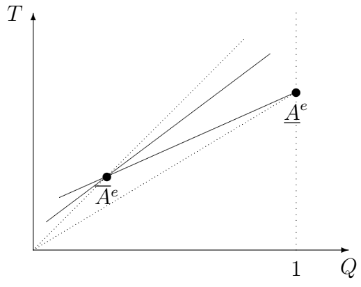
Figure 1 Equilibrium allocations under exclusive competition
