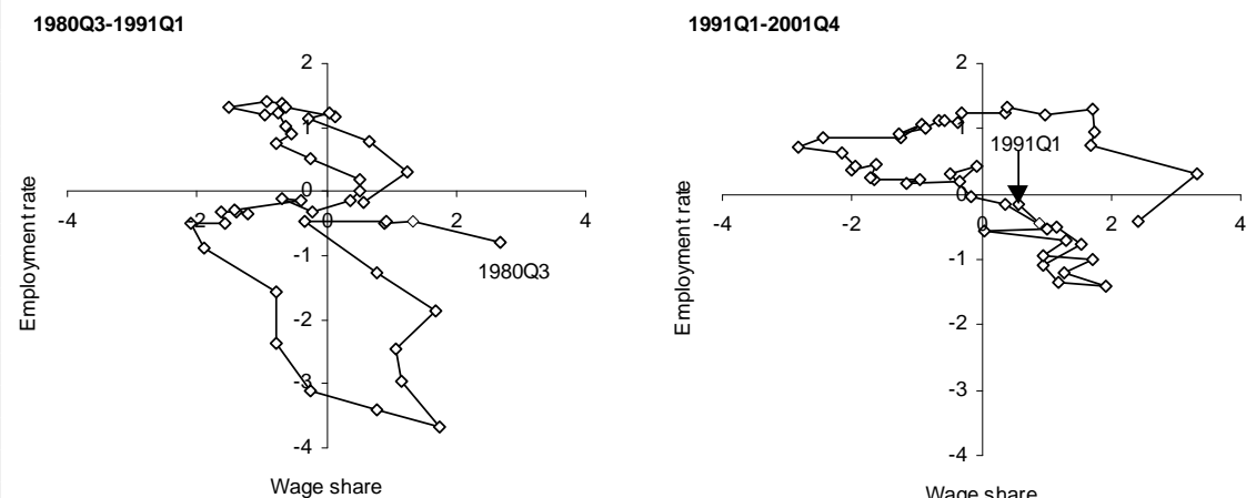
Figure 5: Detrended Corporate Sector Cycles, USA, Quarterly Data, 1980-2001
